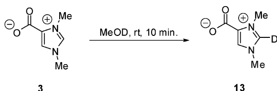
Scheme 6
