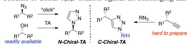
Scheme 1. Chiral 1,2,3-triazole ligand: an challenging task.
