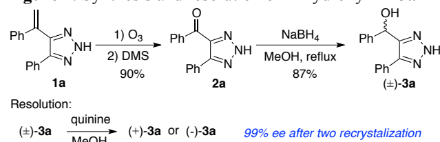
Figure 1. Synthesis and resolution of \alpha -hydroxy TA 3a
