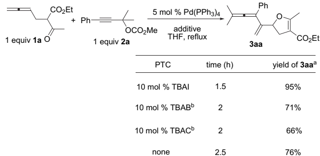
Scheme 2. Effect of tetrabutylammonium halide on the reaction of 1a with 2a .
