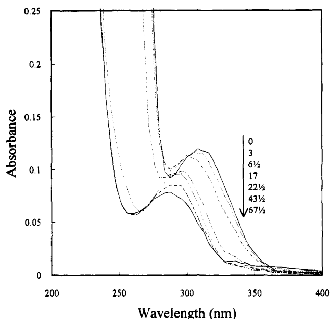
Figure 3. Spectral changes during 254 nm photolysis at 25 °C of 4.0 \times 10^{-4} mol·L ^{-1} carvone in degassed 42% ethanol: UV-visible absorption spectrum prior to light exposure and after 3, 6.5, 17, 22.5, 43.5, and 67.5 h of light exposure ( I_0 = 2.2 \times 10^{17} quanta·s ^{-1} ·L ^{-1} ). Concentrations of carvone, carvonecamphor, and the ester in each of the photolysis solutions are shown in Figure 2.
