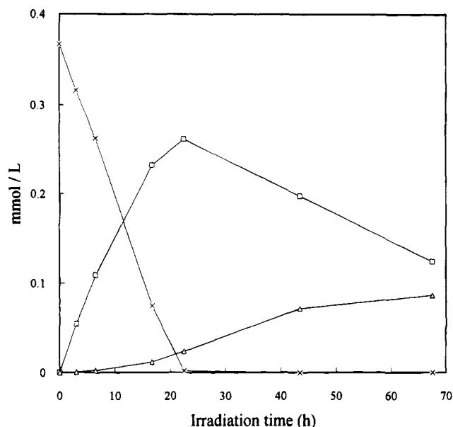
Figure 2. Concentration profile for continuous wave photolysis of 4.0 \times 10^{-4} mol·L ^{-1} carvone in degassed 42% ethanol for 254 nm irradiation ( I_0 = 2.2 \times 10^{17} quanta·s ^{-1} ·L ^{-1} ) at 25 °C based on GC analysis: x, carvone; □, carvonecamphor; Δ, the ester. Absorption spectra of the photolysis solutions are shown in Figure 3.
