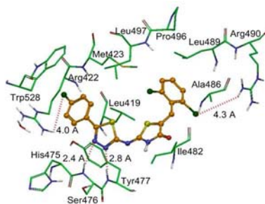
Molecular modeling of compound 24 within the NS5B of HCV.
