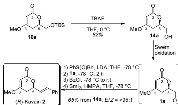
Scheme 6. Total synthesis of ( R )-kavain 2 .
