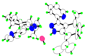
Figure 2. ORTEP of 3-(Pyridin-2'-yl)- l -menthopyrazole ( 1a ).
