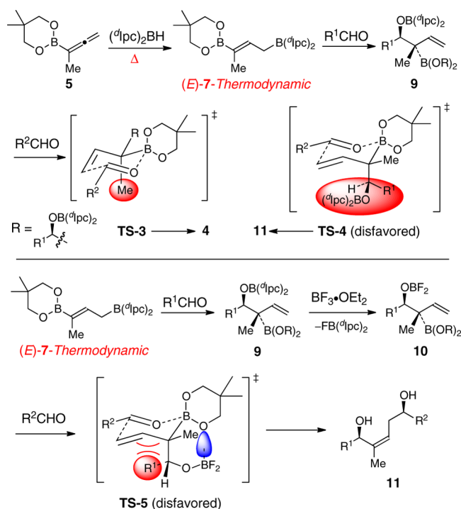
Figure 4. (a) Transition state analyses of second allylboration with allylboronate 9. (b) Transition state analyses of the Lewis acid \text{BF}_3\cdot\text{OEt}_2 catalyzed second allylboration with allylboronate 9.
