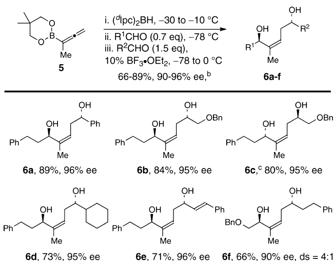
Scheme 2. Synthesis of (Z)-1,5 - anti -Diols 6 via Kinetically Controlled Hydroboration of 5 and the Lewis Acid BF_3 \cdot OEt_2 Catalyzed Double-Allylboration Reactions of Allylborane (Z)-7^a
