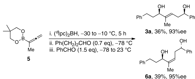
Scheme 1. Initial Attempts at Hydroboration–Double Allylboration with 5
