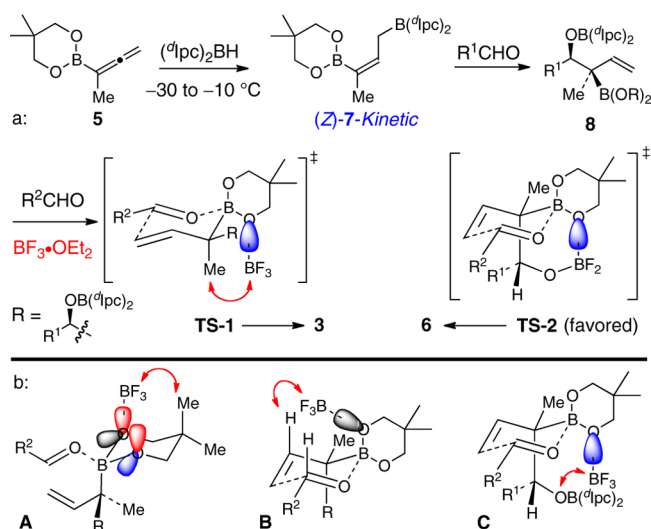
Figure 3. (a) Analysis of transition states for Lewis acid catalyzed second allylboronation with allylboronate 8 . (b) Analyses of the potential interaction of \text{BF}_3 with an oxygen atom in the dioxaborinane unit.
