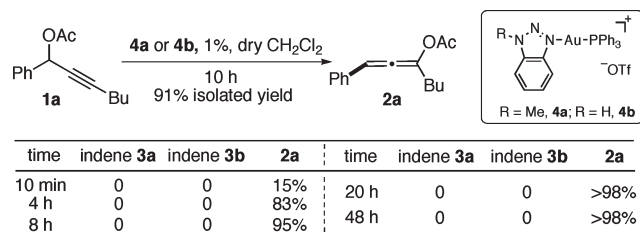
Scheme 3. Proposed \text{S}_{\text{N}}2' Addition Mechanism by Nolan
