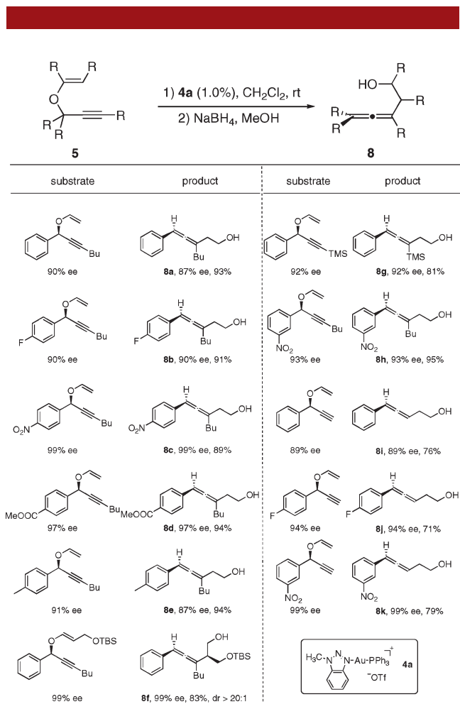
Figure 1. Reaction substrate scope for chiral allenes. General reaction conditions: 5 (0.25 mmol), 4a (1.0%), DCM (2.5 mL), The reactions were monitored by TLC (0.5–12 h), rt; ee was determined by HPLC. For products 8i–j , 4a (3.0%) was used.
