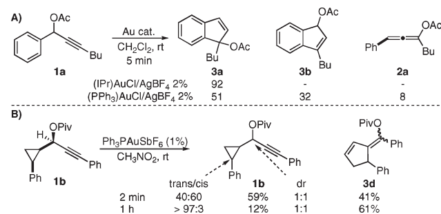
Scheme 2. Trapping the Allene by Proper Synthetic Partners
