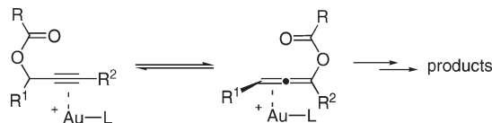
Scheme 1. A Challenge in Cationic Au Catalysis: How to Achieve Chemoselective Activation of Alkyne over Allene?
