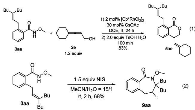
Scheme 2. Axial Chirality Transfer Reactions
