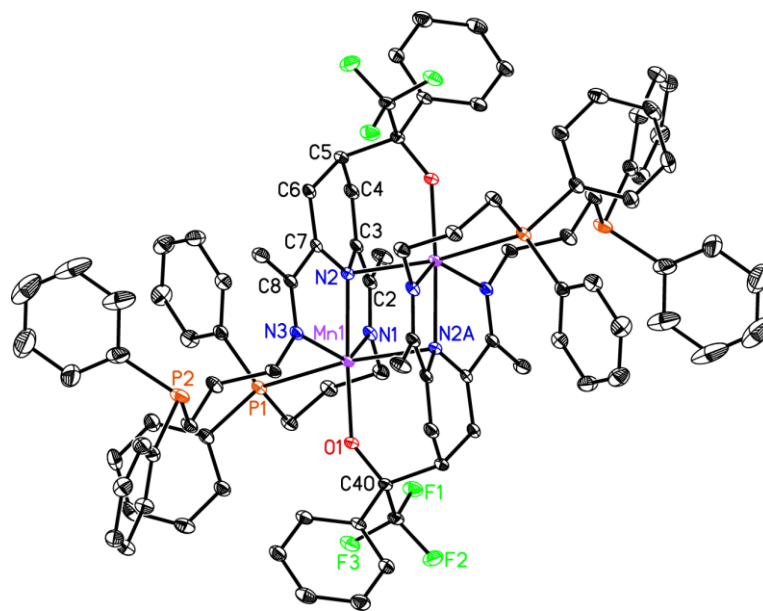
Figure 7. The solid-state structure of 4 shown at 30% probability ellipsoids. Atom labels ending with “A” were generated by symmetry. Hydrogen atoms and three co-crystallized THF molecules per asymmetric unit have been omitted for clarity.
