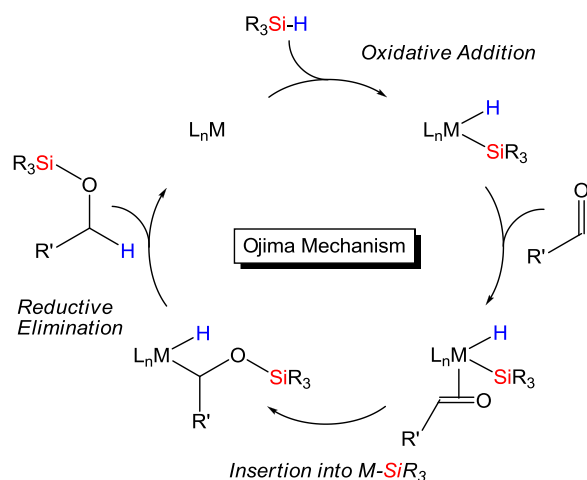
Figure 1. Ojima mechanism for carbonyl hydrosilylation.
