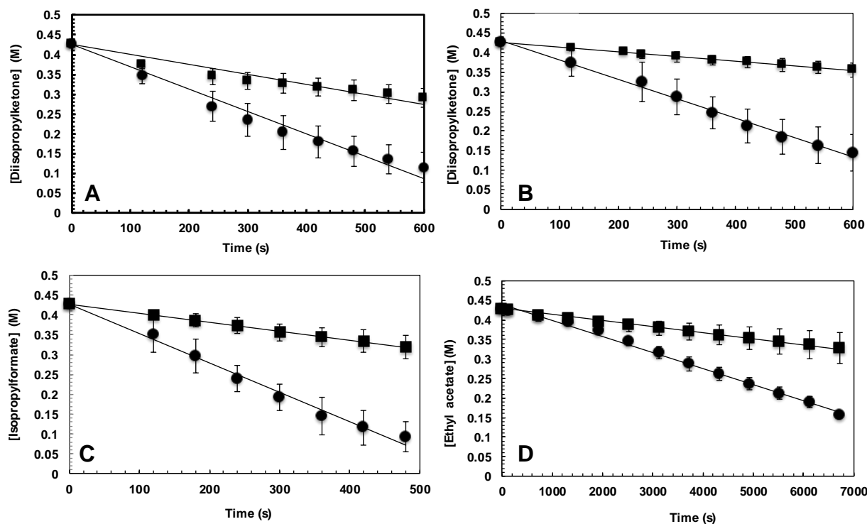
Figure 10. The disappearance of diisopropyl ketone in the presence of \text{PhSiH}_3 (●) and \text{PhSiD}_3 (■) catalyzed by 1.0 mol% 1 (A, \text{KIE} = 2.2 \pm 0.1 ). Rates are 5.654 \times 10^{-4} \text{ M/s} ( \text{PhSiH}_3 ) and 2.534 \times 10^{-4} \text{ M/s} ( \text{PhSiD}_3 ). The disappearance of diisopropyl ketone in the presence of \text{PhSiH}_3 (●) and \text{PhSiD}_3 (■) catalyzed by 1.0 mol% 2 (B, \text{KIE} = 4.1 \pm 0.6 ). Rates are 4.96 \times 10^{-4} \text{ M/s} ( \text{PhSiH}_3 ) and 1.19 \times 10^{-4} \text{ M/s} ( \text{PhSiD}_3 ). Isopropyl formate dihydrosilylation using \text{PhSiH}_3 and 1.0 mol% of 1 (■, 2.26 \times 10^{-4} \text{ M/s} ) and 2 (●, 7.37 \times 10^{-4} \text{ M/s} ) at 25^\circ \text{C} in benzene- d_6 (C). Ethyl acetate dihydrosilylation using \text{PhSiH}_3 and 1.0 mol% of 1 (■, 0.16 \times 10^{-4} \text{ M/s} ) and 2 (●, 0.41 \times 10^{-4} \text{ M/s} ) at 25^\circ \text{C} in benzene- d_6 (D).
