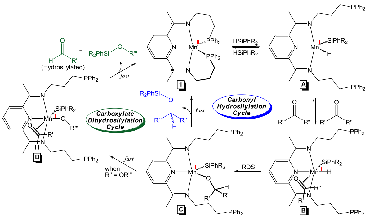
Figure 11. Modified Ojima mechanism for 1 -catalyzed aldehyde ( R' = \text{H} , R'' = \text{alkyl or aryl} ), ketone ( R', R'' = \text{alkyl or aryl} ), formate ( R' = \text{H} , R'' = \text{OR}''' ; where R''' = \text{alkyl} ), and ester ( R' = \text{alkyl} , R'' = \text{OR}''' ; where R''' = \text{alkyl or aryl} ) hydrosilylation.
