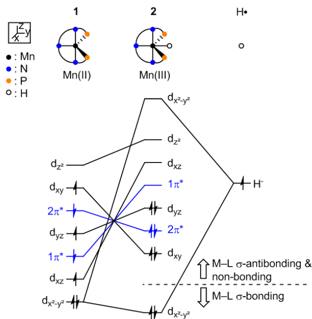
Figure 5. Energy-level diagram for 2 .
