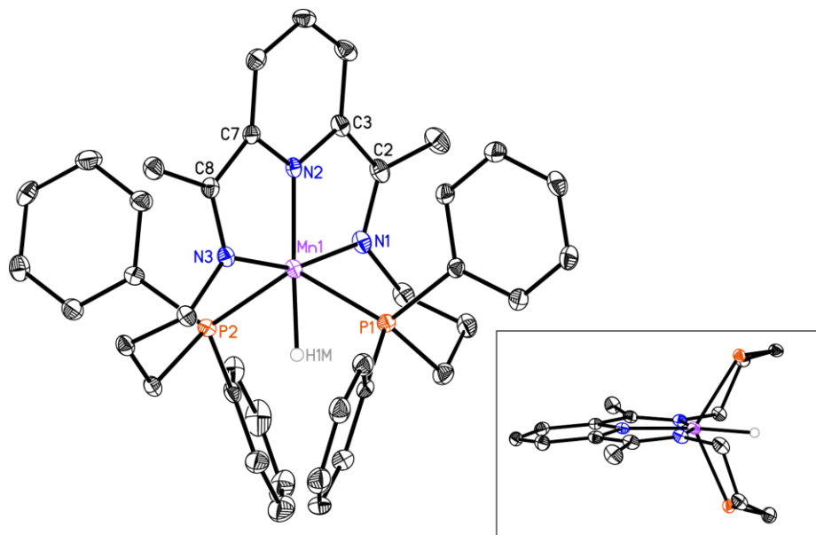
Figure 3. The molecular structure of 2 shown at 30% probability ellipsoids. The asymmetric unit was found to possess a second molecule of 2 , which has been omitted for clarity. Hydrogen atoms other than H1M are also omitted. The inset highlights the capped trigonal bipyramidal geometry about Mn (considering axial imine N atoms) with aryl groups removed for clarity.
