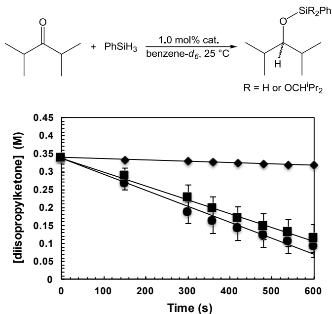
Figure 8. Diisopropyl ketone hydrosilylation at 1.0 mol% catalyst loading in 0.7 mL benzene- d_6 . Rates of 1 (●), 2 (■), and 3 (◆) catalyzed reactions are 4.48 \times 10^{-4} , 3.87 \times 10^{-4} , and 0.36 \times 10^{-4} M/s, respectively.
