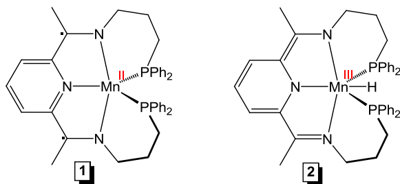
Figure 6. Lewis structure of 1 and 2 most consistent with the computed electronic structures.
