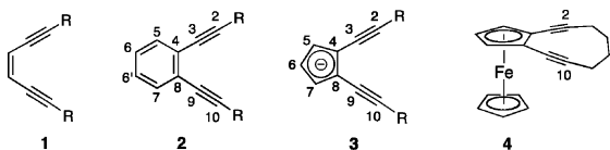
Figure 1. Acyclic enediynes ( 1 ), benzoenediynes ( 2 ), cyclopentadienidoenediynes ( 3 ), and iron enediynes ( 4 ). The numbering used in the text is also shown.
