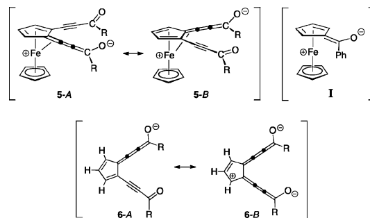
Scheme 1. Resonance Contributors for 5 and 6 and the Proposed 5a Excited State I for Ligand Loss upon Photolysis of \text{CpFe}[\text{C}_5\text{H}_3(\text{COR})_2]
