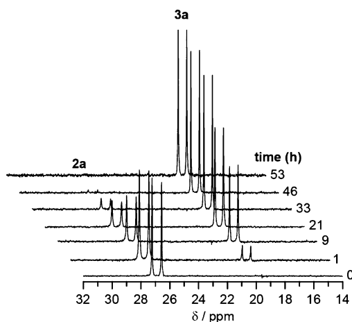
Figure 3. Temporal evolution of the ^{31}\text{P}\{^1\text{H}\} NMR spectra when 2a , in the presence of 2.1 M HCl, is treated with ca. 0.2 atm of \text{O}_2 at room temperature. Spectra were collected at the time intervals depicted on the right of the plot. Resonances attributed to 2a and 3a are labeled.
