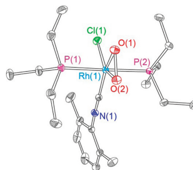
Figure 5. Thermal ellipsoid plot of 4b , shown at the 50% probability level. All hydrogen atoms are omitted for clarity. Data were collected at 100(2) K.
