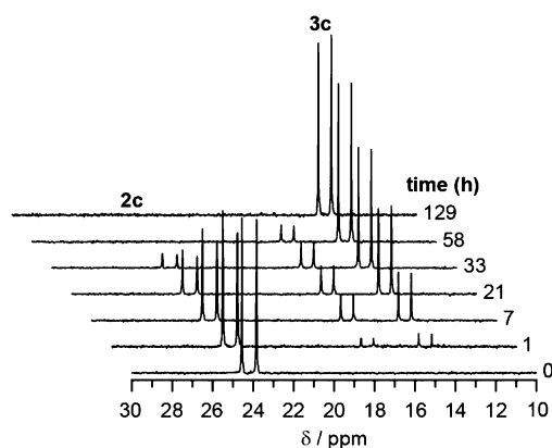
Figure 4. Time-resolved ^{31}\text{P}\{^1\text{H}\} NMR spectra when 2c , in the presence of 77 mM HCl, is treated with 1 atm of \text{O}_2 at room temperature. Spectra were collected at the time intervals depicted on the right of the plot. Resonances attributed to 2c and 3c are labeled.
