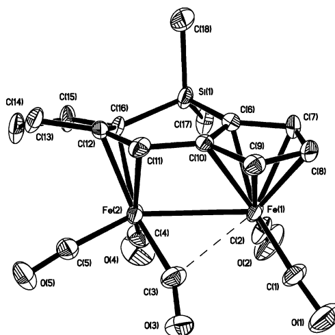
Figure 12. ORTEP diagram of 24 . Thermal ellipsoids are shown at the 30% level. Selected bond lengths (Å) and angles (deg): Fe(1)–Fe(2) = 2.771(2), Fe(1)–C(3) = 2.400(10), Fe(1)–C(6) = 2.106(8), Fe(1)–C(10) = 2.133(7), Fe(2)–C(3) = 1.814(9), Fe(2)–C(11) = 2.095(7), Fe(2)–C(12) = 2.107(7), Fe(2)–C(16) = 2.223(8), Si(1)–C(6) = 1.854(8), Si(1)–C(16) = 1.853(8), C(10)–C(11) = 1.448(10), C(11)–C(12) = 1.406(10), C(12)–C(13) = 1.505(10), C(13)–C(14) = 1.511(12), C(14)–C(15) = 1.512(11), C(15)–C(16) = 1.517(10), C(12)–C(16) = 1.387(10); C(12)–C(11)–C(10) = 120.7(7), C(16)–C(12)–C(11) = 122.7(7), C(6)–Si(1)–C(16) = 98.7(4), O(1)–C(1)–Fe(1) = 176.4(10), O(2)–C(2)–Fe(1) = 175.5(8), O(3)–C(3)–Fe(1) = 122.2(7), O(3)–C(3)–Fe(2) = 156.9(8), O(4)–C(4)–Fe(2) = 175.9(9), O(5)–C(5)–Fe(2) = 175.1(8).
