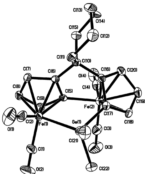
Figure 11. ORTEP diagram of 21 . Thermal ellipsoids are shown at the 30% level. Selected bond lengths (Å) and angles (deg): Ge(1)–Fe(1) = 2.3749(10), Fe(1)–C(6) = 2.116(4), Fe(1)–C(5) = 2.159(4), Fe(2)–C(5) = 1.977(5), Fe(2)–C(16) = 2.077(4), Fe(2)–C(17) = 2.096(4), Ge(1)–C(17) = 1.968(4), C(6)–C(10) = 1.508(6), C(10)–C(16) = 1.536(6); C(17)–Ge(1)–Fe(1) = 103.79(13), Fe(2)–C(5)–Fe(1) = 129.2(2), C(6)–C(10)–C(16) = 103.3(3).
