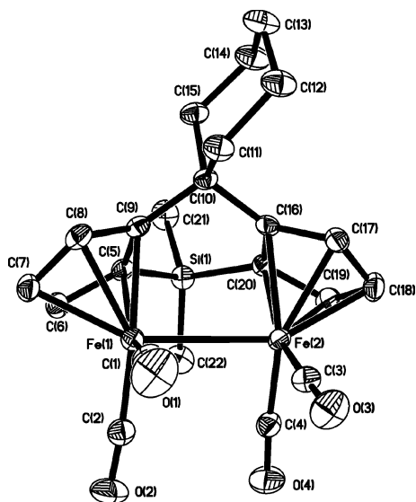
Figure 10. ORTEP diagram of 18 . Thermal ellipsoids are shown at the 30% level. Selected bond lengths (Å) and angles (deg): Fe(1)–Fe(2) = 2.7522(9), Fe(1)–C(5) = 2.117(3), Fe(1)–C(9) = 2.103(3), Fe(2)–C(16) = 2.131(3), Fe(2)–C(20) = 2.116(3), Si(1)–C(5) = 1.866(3), Si(1)–C(20) = 1.863(3), C(10)–C(9) = 1.519(4), C(10)–C(16) = 1.524(4); C(9)–C(10)–C(16) = 106.5(2), C(5)–Si(1)–C(20) = 95.42(12).
