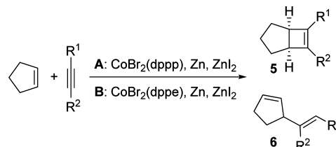
Scheme 3. Cobalt-Catalyzed Alder–Ene Reaction or [2 + 2] Cycloaddition of Cyclopentene with Unsymmetrical Alkynes
