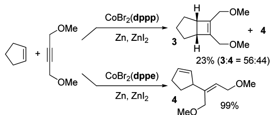
Scheme 2. Cobalt-Catalyzed [2 + 2] Cycloaddition and Alder–Ene Reaction with 1,4-Dimethoxybut-2-yne as Substrate
