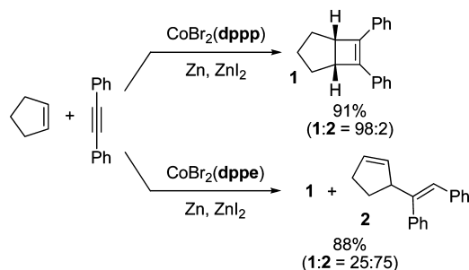
Scheme 1. Cobalt-Catalyzed [2 + 2] Cycloaddition and Alder–Ene Reaction with Diphenyl Acetylene as Substrate
