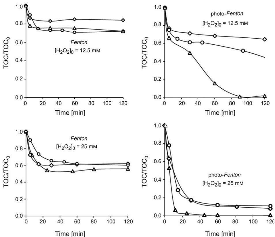
Fig. 5. Evolution of TOC during the oxidative degradation of 2,4-DHBA in aqueous solution by the Fenton and photo- Fenton processes under different conditions of oxygenation. \diamond : air-equilibrated solution; \circ : air-saturated solution; \triangle : \text{O}_2 -saturated solution; [\text{H}_2\text{O}_2]_0 = 12.5 mM or 25 mM, [\text{Fe}^{\text{II}}]_0 = 0.5 mM, [\text{TOC}]_0 = 218 mg \text{l}^{-1} ( [2,4\text{-DHBA}]_0 = 2.6 mM).
