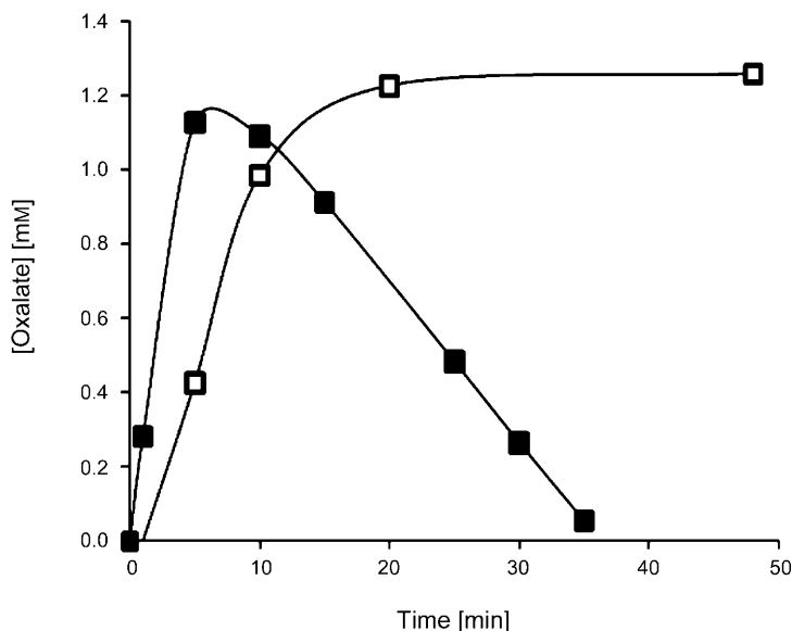
Fig. 7. Evolution of the concentration of oxalic acid during the oxidative degradation of 2,4-DHBA in air-saturated aqueous solutions by the Fenton (□) and photo-Fenton (■) processes. [\text{Fe}^{\text{II}}]_0 = 0.5 \text{ mM} , [\text{H}_2\text{O}_2]_0 = 25 \text{ mM} , and [2,4\text{-DHBA}]_0 = 2.6 \text{ mM} .
