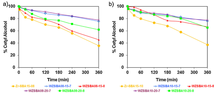
Fig. 5. Catalytic results for the esterification of cetyl alcohol and palmitic acid over (a) Zr-SBA15-08 and (b) Zr-SBA15-10 based catalysts.
