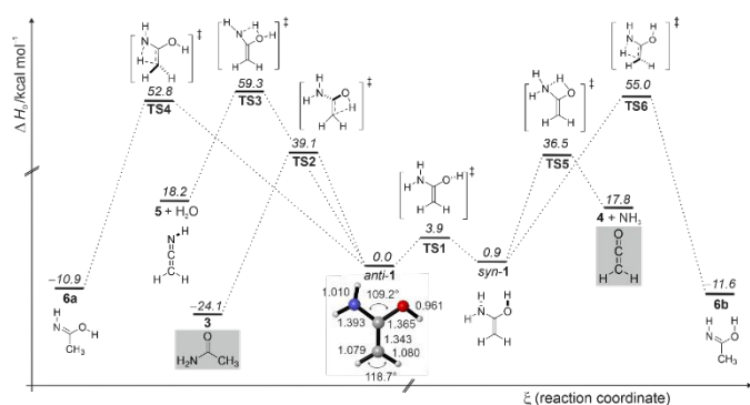
Figure 3. Potential energy profile ( \Delta H_0 ) in \text{kcal mol}^{-1} of the reactions of enol 1 at AE-CCSD(T)/cc-pVTZ + ZPVE at 0 K.
