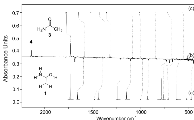
Figure 1. IR spectrum showing the pyrolysis product of 2 with subsequent trapping in an argon matrix at 10 K. (a) IR spectrum of 1 computed at AE-CCSD(T)/cc-pVTZ (unscaled). (b) IR difference spectrum showing the photochemistry of 1 after irradiation with \lambda > 270 \text{ nm} in argon at 10 K. Downward bands assigned to 1 disappear while upward bands assigned to 3 and 4 appear after 30 min irradiation time. (c) IR spectrum of 3 computed at AE-CCSD(T)/cc-pVTZ (unscaled).
