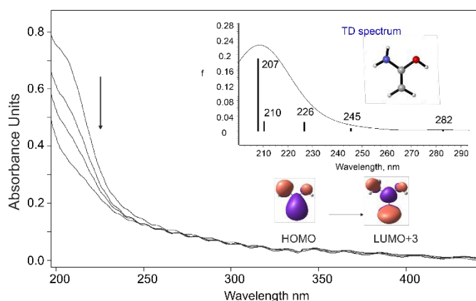
Figure 2. Solid line: UV/Vis spectrum of 1 isolated at 10 K in Ar. Dashed lines: the photochemistry of 1 after irradiation at \lambda > 270 \text{ nm} for 1, 5, and 15 min in argon at 10 K. Inset: computed [TD-B3LYP/6-311++G(2d,2p)] electronic transitions for 1 .
