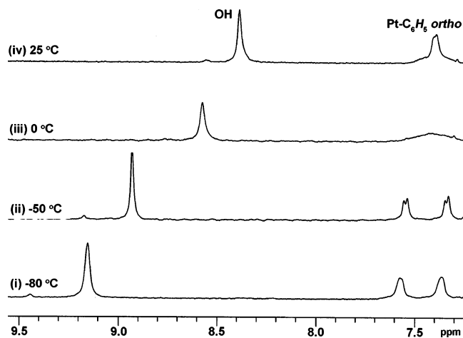
Figure 2. Variable-temperature ^1\text{H} NMR spectra of 1a in toluene- d_8 at (i) -80 ^\circ\text{C} , (ii) -50 ^\circ\text{C} , (iii) 0 ^\circ\text{C} , and (iv) 25 ^\circ\text{C} .
