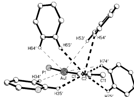
Figure 2. (Top) Molecular structure of 10 (50% thermal ellipsoids). (Bottom) Clustering of \text{C-H}\cdots\text{Au} (thin dashed bonds) and \text{C-H}\cdots\pi contacts (thick dashed bonds) at the \text{P-Au-C}\equiv\text{C} center of compound 10 . For symmetry operators, see Supporting Information.
