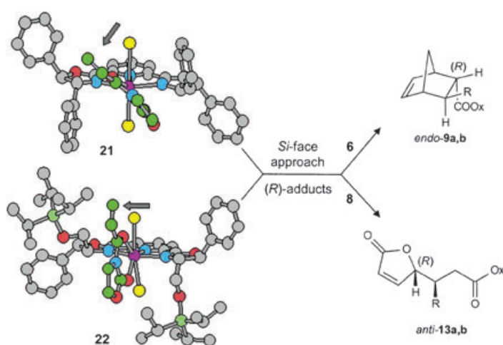
Figure 5. Assumed reactive intermediates for the reactions of 5 with both 6 (Diels–Alder) and 8 (Mukaiyama–Michael), catalysed by the \text{La}(\text{OTf})_3 complexes of pybox 16 (reactive intermediate 21 ) and 4 (reactive intermediate 22 ).
