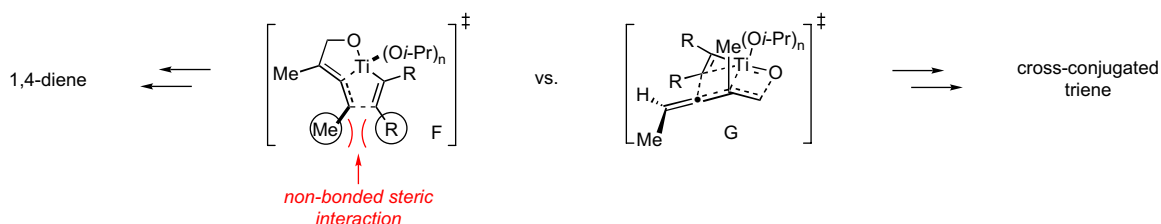
Figure 3. Competition between directed carbometallation and formal metallo-[3,3] rearrangement with trisubstituted allenes.
