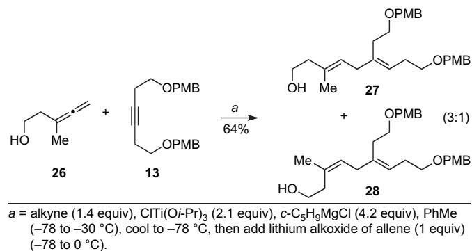
Scheme 6. Cross-coupling of homoallenic alcohols with alkynes leads to diminished stereoselection.
