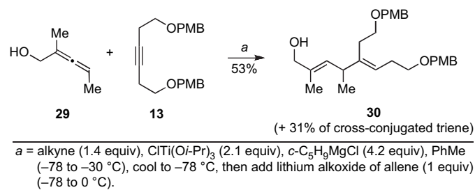
Scheme 7. Cross-coupling of trisubstituted allenes with internal alkynes.
