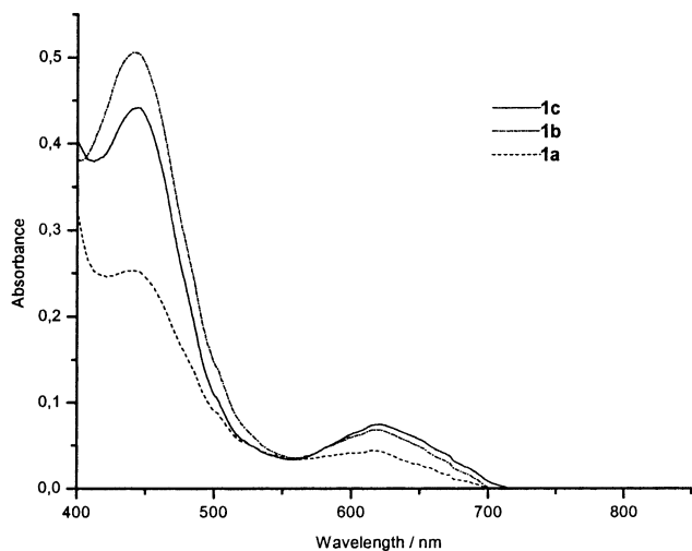
Fig. 1. Electronic absorption spectra of 1a–c in dichloromethane ( c = 5 \times 10^{-4} M).
