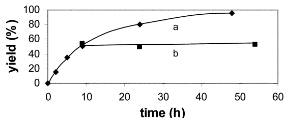
Fig. 2 Time conversion plot for the room temperature Baylis–Hillman reaction of 4-nitrobenzaldehyde (1 equiv.) and methyl vinyl ketone (3 equiv.) in DMF (5 mL) in the presence of solid catalyst (1 equiv.) (a) and after filtering the solid at 50% conversion (b).
