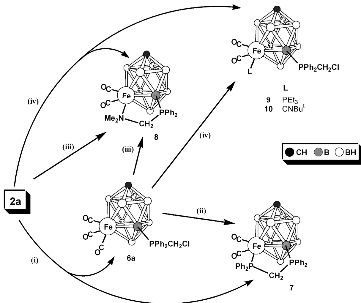
Scheme 1. Formation and Interconversion of Compounds 6a and 7–10 from 2a a
