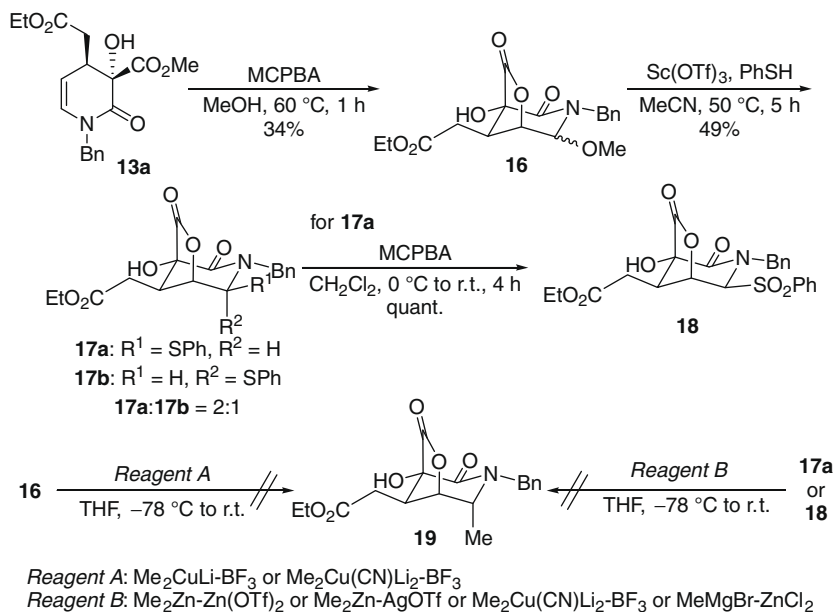
Scheme 4.
