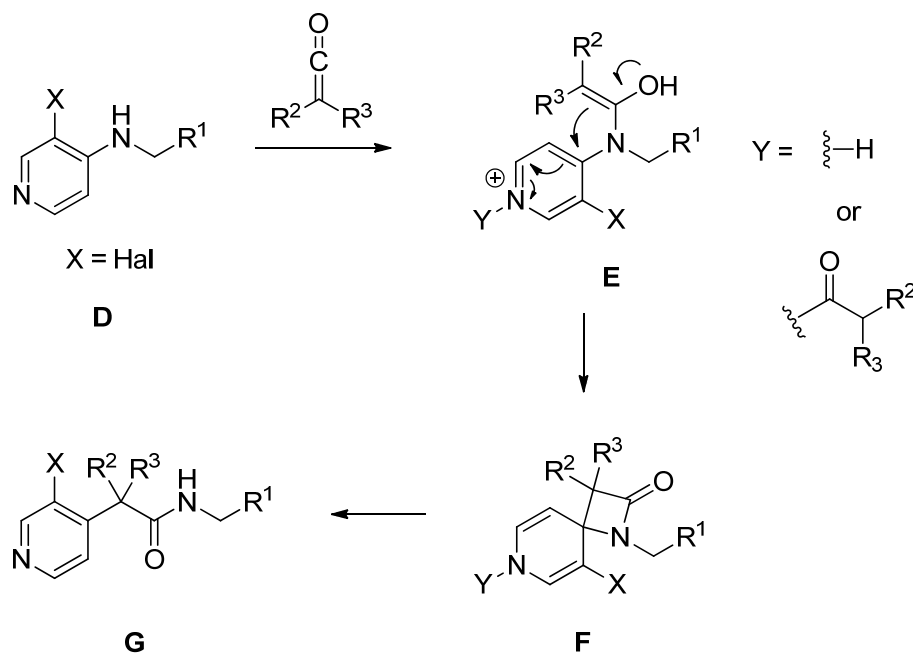
SCHEME 2. Proposed mechanism for the rearrangement of 4-amino-3-halo-pyridines
