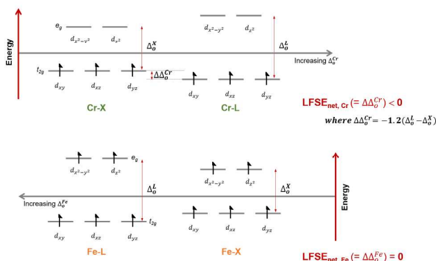
Figure 5. Analysis of the orbital interaction contribution to \Delta H_{\text{sys}} using ligand field theory with a simplified coordination environment ( O_h ) for the metal metathesis process in PCN-333.
