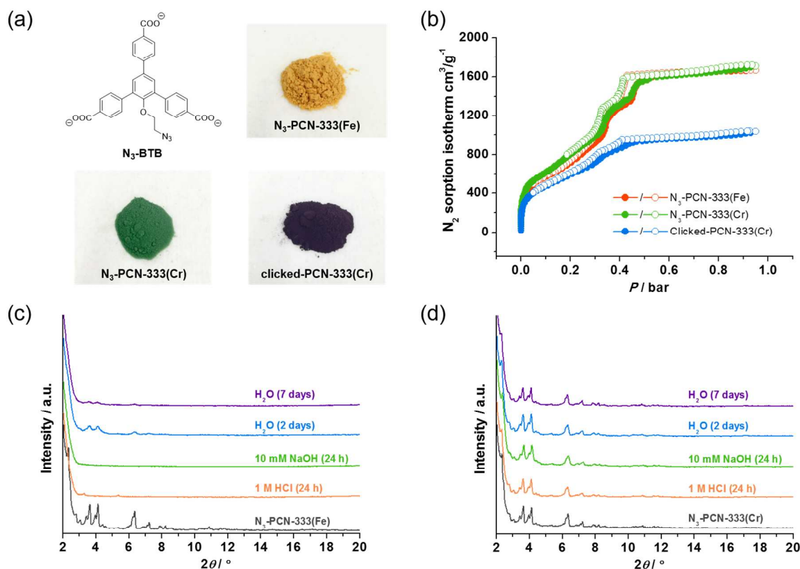
Figure 6. (a) N_3 -BTB used for ligand exchange and photographs of N_3 -PCN-333(Fe), N_3 -PCN-333(Cr), and N_3 -PCN-333(Cr) after click reaction. (b) N_2 sorption isotherm of N_3 -PCN-333(Fe), N_3 -PCN-333(Cr), and N_3 -PCN-333(Cr) after click reaction. (c) PXRD patterns of N_3 -PCN-333(Fe) and (d) N_3 -PCN-333(Cr) after different treatments.
