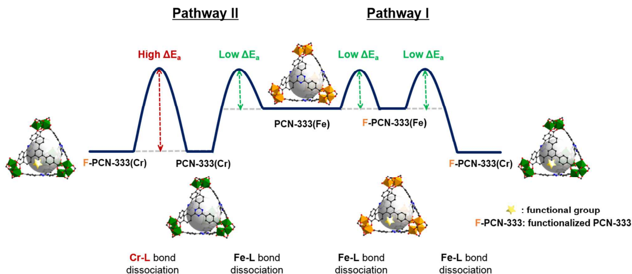
Scheme 1. The energy diagrams of two possible dual exchange routes to functionalized PCN-333(Cr).
