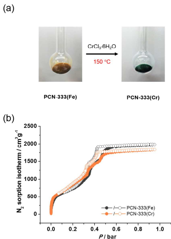
Figure 3 (a) Photographs of PCN-333(Fe) and PCN-333(Cr) exchanged at 150^\circ\text{C} . (b) \text{N}_2 sorption isotherm of PCN-333(Fe) and PCN-333(Cr) at 77 K.
