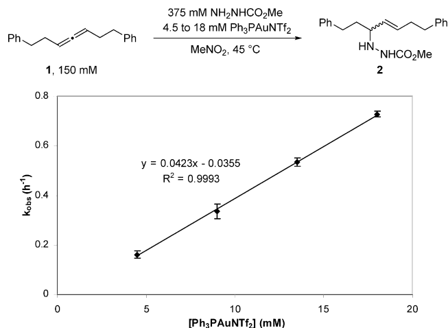
Figure 5. A plot of k_{\text{obs}} versus [\text{Ph}_3\text{PAuNTf}_2] , using 2.5 equiv of methyl carbazate.
