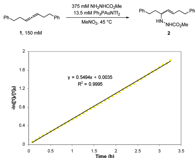
Figure 4. A representative plot of -\ln([1]/[1]_0) versus time (h) for the reaction of 1 and methyl carbazate shows first-order dependence in 1 .
