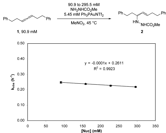
Figure 3. A plot of k_{\text{obs}} versus concentration of methyl carbazate, where k_{\text{obs}} was determined by the method of initial rates.
