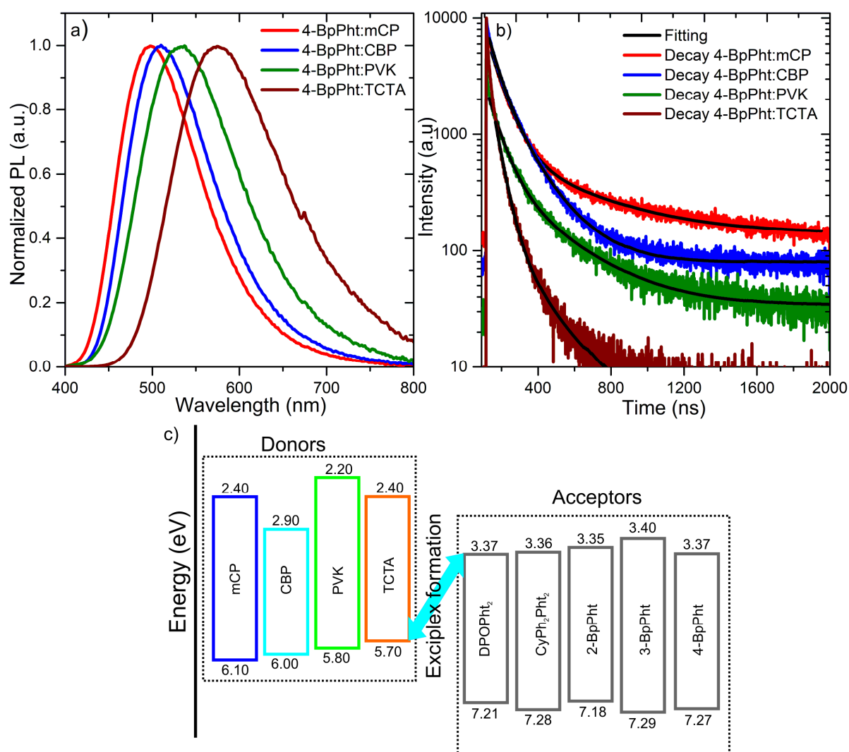
Figure 7. PL spectra (a) and PL decay curves (b) of the layers of blends: 4-BpPht:mCP, 4-BpPht:CBP, 4-BpPht:PVK and 4-BpPht:TCTA. Schematic representation of energy band diagrams of exciplex-forming carbazole-based donors and phthalimide acceptors (c).
