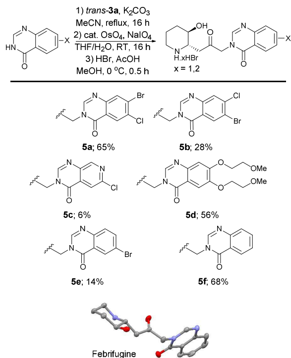
Scheme 3. Synthesis of quinazolinones by directed CH -amidation.
