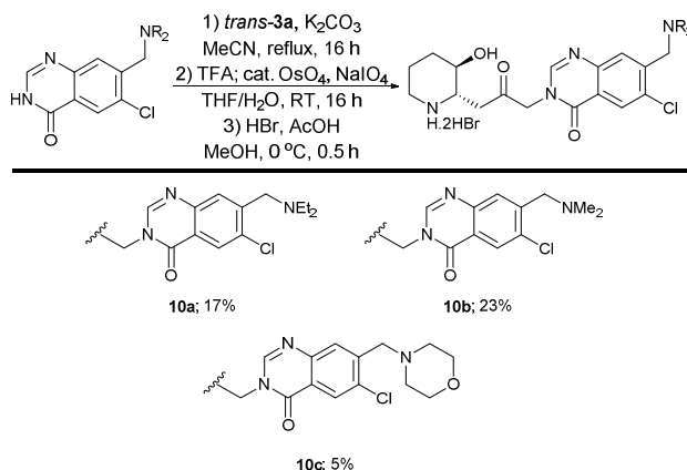
Scheme 7. Synthesis of amino-methyl febrifugine analogs.
