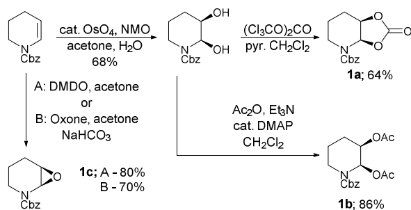
Scheme 2. Synthesis of functionalized piperidines.
