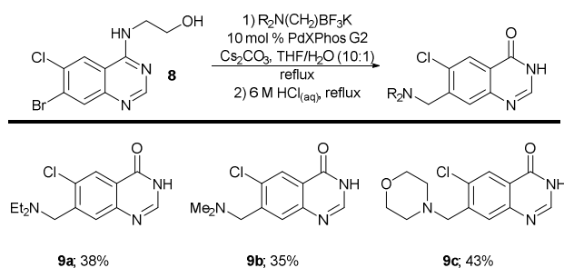
Scheme 6. Synthesis of amino-methyl functionalized quinazolinones.
