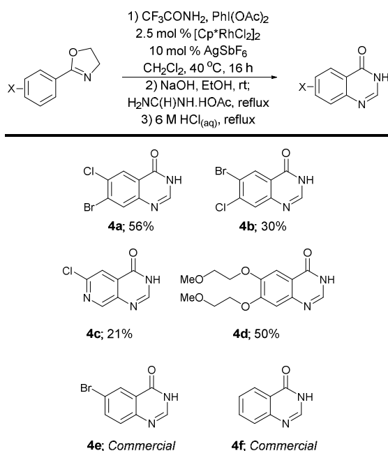
Scheme 3. Synthesis of quinazolinones by directed CH -amidation.
