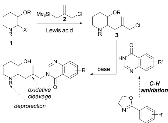
Scheme 1. Convergent route to febrifugine analogs.
