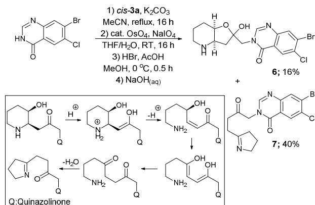
Scheme 5. Investigation towards the synthesis of the iso-febrifugines.
