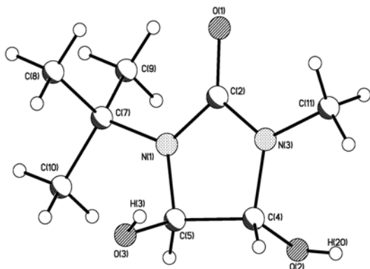
Figure 4. General view of 11c . Selected bond lengths(Å): N(1)-C(2) 1.368(3), N(1)-C(5) 1.452(3), O(1)-C(2) 1.228(3), O(2)-C(4) 1.409(3), O(3)-C(5) 1.409(3), C(2)-N(3) 1.358(3), N(3)-C(4) 1.433(3); bond angles(°): C(2)-N(1)-C(5) 109.7(2), C(2)-N(1)-C(7) 123.7(2), C(5)-N(1)-C(7) 124.4(2), O(1)-C(2)-N(3) 125.1(2), O(1)-C(2)-N(1) 126.4(2), N(3)-C(2)-N(1) 108.4(2), C(2)-N(3)-C(4) 111.2(2), C(2)-N(3)-C(11) 123.2(2), C(4)-N(3)-C(11) 124.4(2).
