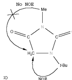
Figure 2. Difference mode NOE experiments of 13c in \text{DMSO-d}_6
