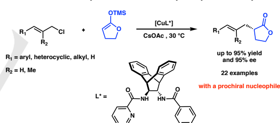
Figure 1. Transition-metal catalyzed \alpha -alkylation of \gamma -butyrolactones.
