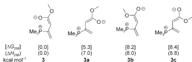
Figure 4. DFT-computed relative enthalpies and free energies of four possible structures of the 1,3-dipole generated from PMe 3 and allenolate.
