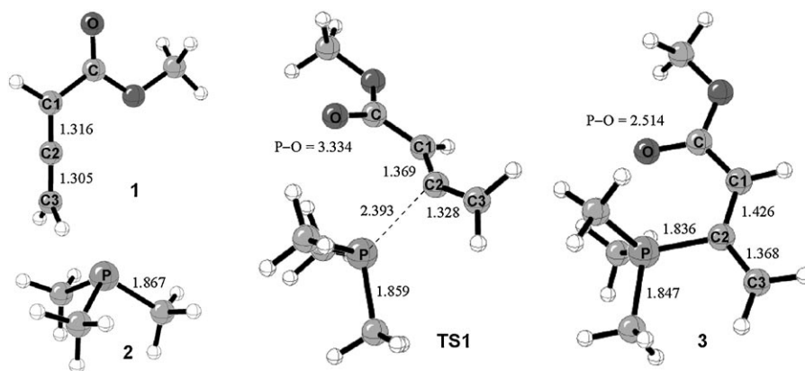
Figure 2. DFT-optimized structures of 1 , 2 , transition state TS1 , and 1,3-dipole 3 . Distances are in Å.
