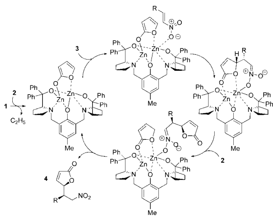
Scheme 1. Proposed Catalytic Cycle
