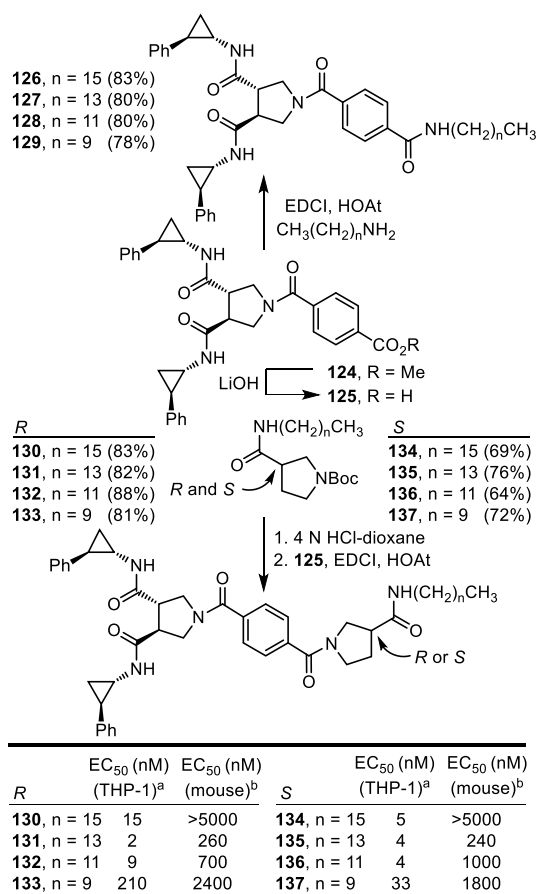
Figure 14. Hybrid structures containing one lipid side chain and a total of three hydrophobic amide side chains. EC 50 's derived from dose-response curves for the stimulated release of TNF-α from differentiated human THP-1 cells or mouse macrophages.
