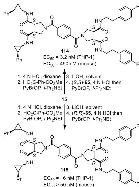
Figure 12. Diprovocim-4 and diprovocim-5. EC 50 's derived from dose-response curves for the stimulated release of TNF-α from differentiated human THP-1 cells or mouse macrophages.
