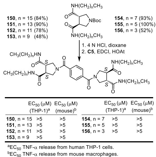
Figure 16. Compounds that contain a full set of four lipid chain amides.
