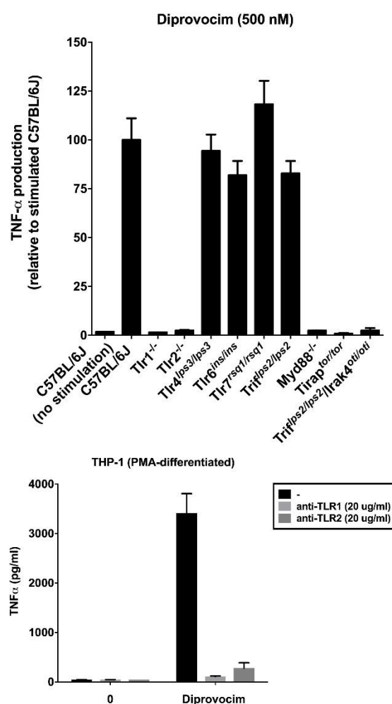
Figure 18. Top: Assay for stimulated TNF- \alpha release upon treatment with 3 (500 nM) using macrophages from mice containing disabling germline mutations or knockouts of genes encoding key mTLRs and downstream signaling proteins. Bottom: Assay for stimulated TNF- \alpha release upon treatment with 3 (250 pM) versus controls without compound using differentiated THP-1 cells that is blocked by antibodies that bind either TLR1 or TLR2. All results are representative of two independent experiments and error bars represent SEM.
