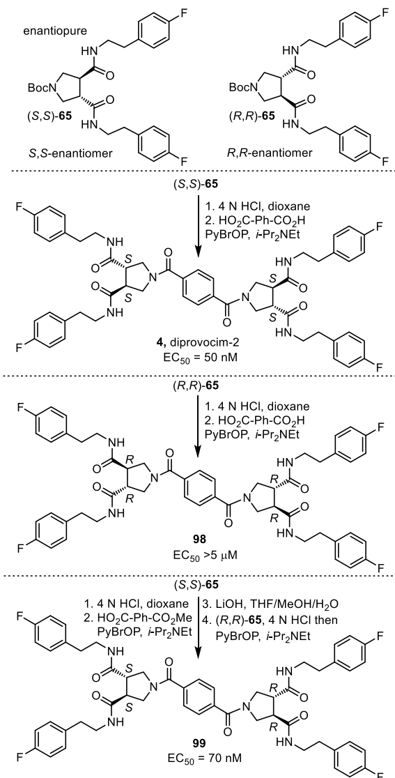
Figure 10. Synthesis of the three enantiopure compounds found in the all racemate 69 , identifying the active components. EC_{50} 's were derived from dose-response curves for the stimulated release of TNF- \alpha from differentiated human THP-1 cells by 4 (diprovocim-2) and 98–99 .
