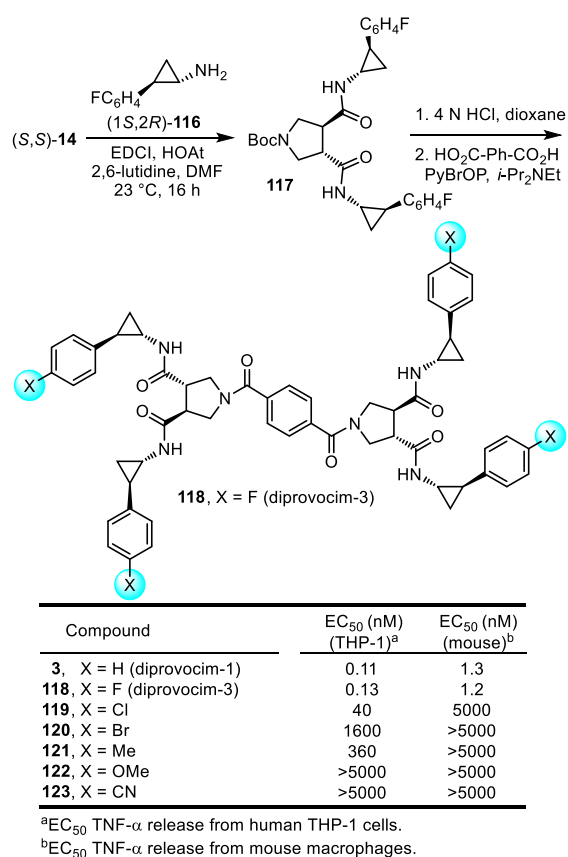
Figure 13. Diprovocim-3 ( 118 ) and related aryl substitution analogues 119–123 of diprovocim-1 ( 3 ).
