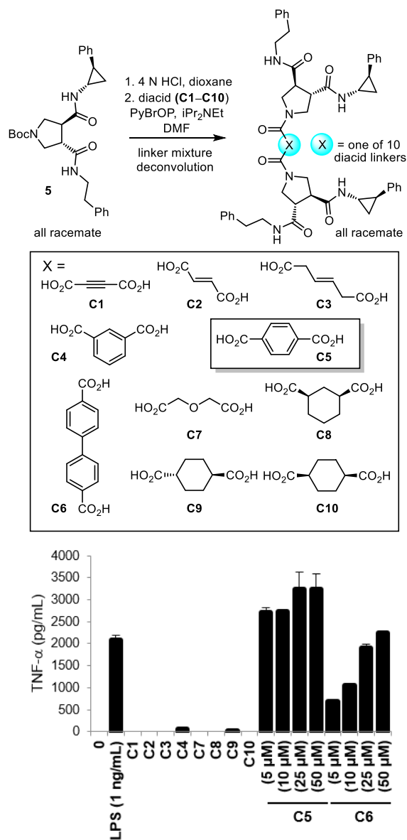
Figure 3. Top: Synthesis of the individual compounds in plate 39G9 used to identify the linker of active compounds. Bottom: Activity of individual compounds (labeled by the linker C1 – C10 ) in the plate 39G9 mixture of the receptor dimerization library tested alongside controls (LPS and 0 = no compound) measuring stimulated TNF- \alpha release from differentiated human THP-1 cells (tested at 50 \mu M unless indicated otherwise).
