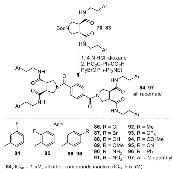
Figure 9. Aryl substituent effects on activity of diprovocim-2 ( 4 ).
