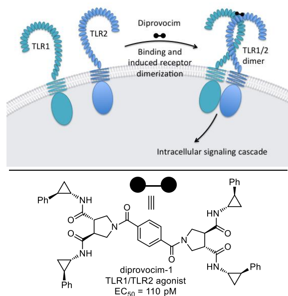
Figure 19. One half of diprovocim each binds a receptor protein, promoting receptor dimerization and activation.
