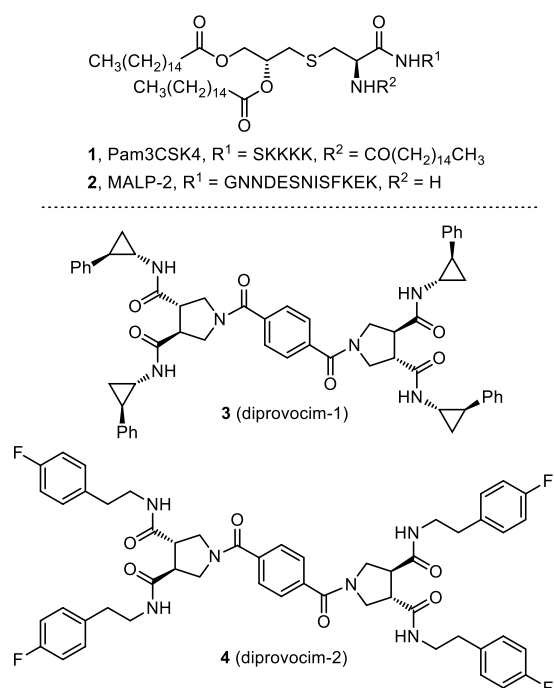
Figure 1. Structures of the known TLR1/TLR2 (Pam3CSK4) and TLR2/TLR6 (MALP-2) agonists and diprovocim-1 and diprovocim-2.
