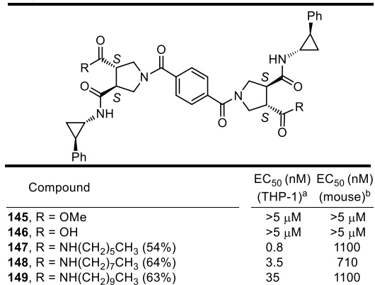
Figure 15. Hybrid structures containing two lipid side chains and a total of four hydrophobic amide side chains.
