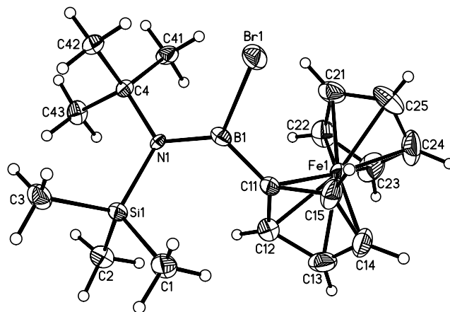
Fig. 2. Molecular structure and numbering scheme of compound 4 . Thermal ellipsoids are shown at the 50% probability level. Selected bond lengths (Å), angles (°) and torsion angles (°) of 4 : B(1)–N(1) = 1.434(7), B(1)–C(11) = 1.518(9), B(1)–Br(1) = 2.003(6), N(1)–C(4) = 1.517(6), N(1)–Si(1) = 1.772(4); C(11)–B(1)–Br(1) = 113.2(4), C(11)–B(1)–N(1) = 125.1(5), N(1)–B(1)–Br(1) = 121.6(4), B(1)–N(1)–Si(1) = 116.5(3), B(1)–N(1)–C(4) = 121.2(4); C(12)–C(11)–B(1)–N(1) = 27.2(8), C(12)–C(11)–B(1)–Br(1) = –154.4(4), C(11)–B(1)–N(1)–C(4) = –142.6(5), C(11)–B(1)–N(1)–Si(1) = 48.1(6), Br(1)–B(1)–N(1)–C(4) = 39.1(6), Br(1)–B(1)–N(1)–Si(1) = –130.2(3).
