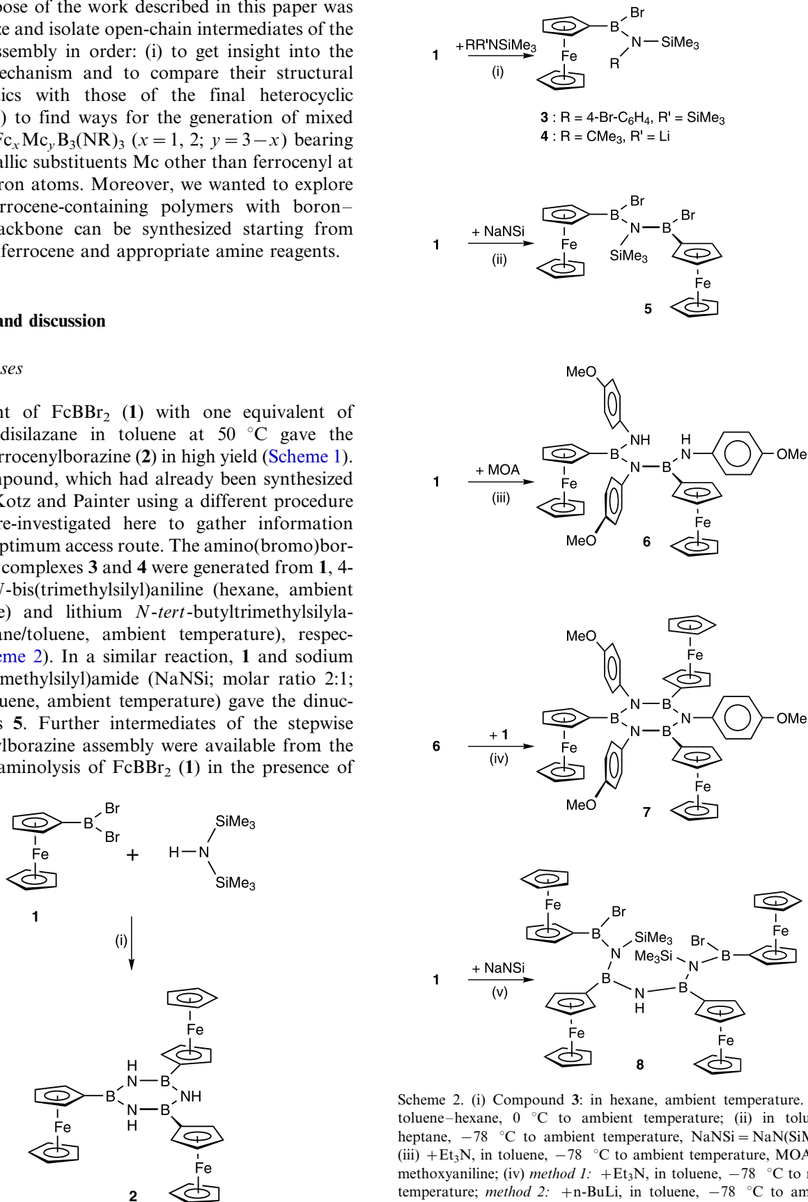
Scheme 1. (i) In toluene, 0–50 °C.
