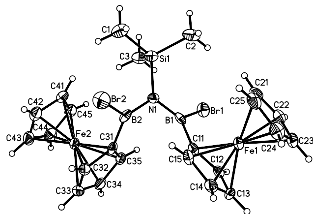
Fig. 3. Molecular structure and numbering scheme of compound 5 . Thermal ellipsoids are shown at the 50% probability level. Selected bond lengths (Å) angles (°) and torsion angles (°) of 5 : B(1)–N(1) = 1.426(6), B(2)–N(1) = 1.447(6), B(1)–C(11) = 1.530(7), B(2)–C(31) = 1.526(7), B(1)–Br(1) = 1.979(5), B(2)–Br(2) = 1.965(5), N(1)–Si(1) = 1.804(4); N(1)–B(1)–C(11) = 125.4(4), N(1)–B(2)–C(31) = 123.0(4), B(1)–N(1)–Si(1) = 121.7(3), B(2)–N(1)–Si(1) = 123.6(3), B(1)–N(1)–B(2) = 114.0(4), C(11)–B(1)–Br(1) = 114.2(3), C(31)–B(2)–Br(2) = 115.7(3); Si(1)–N(1)–B(1)–C(11) = 152.2(3), Si(1)–N(1)–B(2)–C(31) = 124.2(4), Si(1)–N(1)–B(1)–Br(1) = –28.5(5), Si(1)–N(1)–B(2)–Br(2) = –59.2(5), C(11)–B(1)–N(1)–B(2) = –37.1(6), C(31)–B(2)–N(1)–B(1) = –46.2(6), Br(1)–B(1)–N(1)–B(2) = 142.1(3), Br(2)–B(2)–N(1)–B(1) = 130.3(4).
