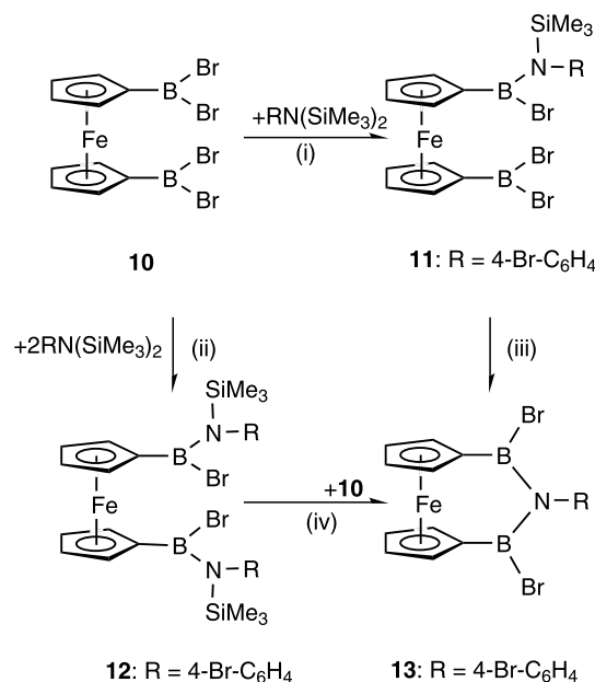
Scheme 4. (i) In toluene, -78^\circ\text{C} to ambient temperature; (ii) in toluene, ambient temperature; (iii) in toluene, reflux temperature; (iv) in toluene, -78^\circ\text{C} to reflux temperature.
