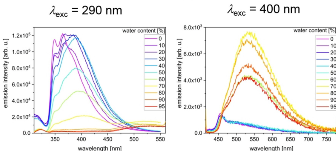
Figure 5. Emission spectra of 4h in ethanol/water upon increasing water content (recorded at T = 298 K, c = 10^{-7} M, \lambda_{\text{exc}} ( 4h ) = 290 nm (left), \lambda_{\text{exc}} ( 4h ) = 400 nm (right); bottom: Emission spectra of 4t in ethanol/water upon increasing water content (recorded at T = 298 K, c = 10^{-7} M, \lambda_{\text{exc}} ( 4t ) = 290 nm (left), \lambda_{\text{exc}} ( 4t ) = 400 nm (right)).
