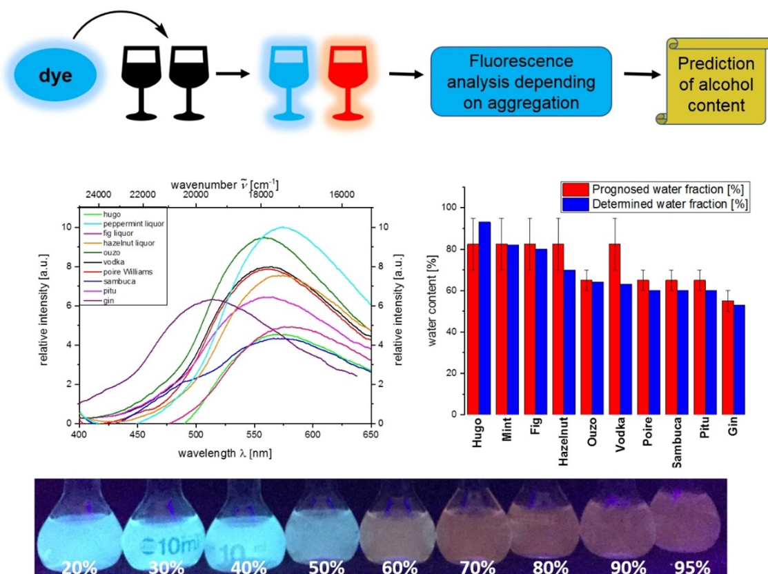
Figure 6. Top: Graphical illustration of alcohol content analysis; Middle, left: Emission spectra of 4h in different alcohols (recorded at T = 298 K, c(\mathbf{4h}) = 10^{-7} M, \lambda_{\text{exc}} = 400 nm); Middle, right: Comparison between prognosed and determined water fraction; Bottom: Visual impression of 4h in ethanol/water mixtures with increasing water content ( \lambda_{\text{exc}} = 365 nm).
