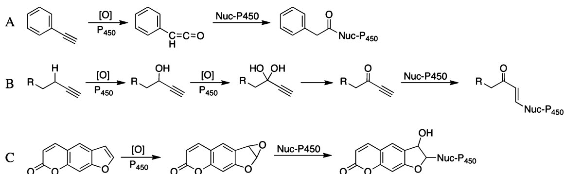
Figure 2. Modes of mechanism-based inactivation of cytochrome P450 enzymes. (A) Aryl alkynes are oxidized to reactive ketene intermediates that inactivate P450s by covalent adduction to the apoprotein. (B) Propynyl-bearing inhibitors are oxidized to a reactive Michael acceptor and inactivate P450s by covalent adduction to the heme or apoprotein. (C) Furanocoumarin inhibitors are oxidized to the reactive furan epoxide and form covalent adducts to the P450 apoprotein.
