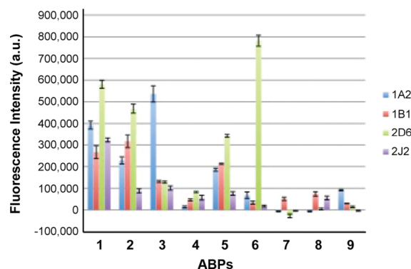
Figure 4. Extracted quantitative data from SDS-PAGE gels of probe labeling, measured as fluorescence intensity (au, arbitrary units). The reported fluorescence intensity values correspond to measurements of P450 bands observed in the gel lanes containing NADPH minus the equivalent size regions of gel lanes lacking NADPH samples. These measurements were restricted to well-defined boundaries around the fluorescence band signals. Data represent the average \pm standard error of three independent experiments per P450 for each ABP. See Supporting Information Figure 4 for quantitative analysis of labeling profiles for the entire 14-member P450 panel.
