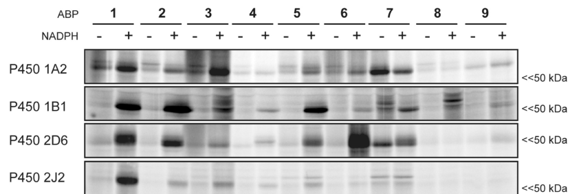
Figure 3. Probe suite labeling of four representative members of the 14-member P450 panel. Full SDS-PAGE separation was performed, but only the 45–55 kDa region is shown, where NADPH-dependent probe-labeled proteins were detected (consistent with the molecular masses of P450 enzymes). See Supporting Information Figure 3 for labeling profiles of the entire 14-member P450 panel. Fluorescent gel shown in grayscale.
