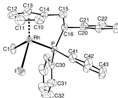
Fig. 1. Displacement ellipsoid plot of ( S Rh , S C )- 6a (Platon98, A.L. Spek, University of Utrecht; 50% probability, H atoms omitted).
