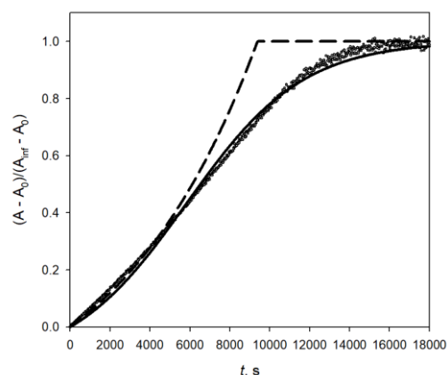
Figure 5 Plot of the normalized absorbance at \lambda = 315 nm for the reaction between 1.0 mM 2 and 0.9 mM fuel 1,H in the presence of 0.1 mM TFA in \text{CH}_2\text{Cl}_2 at 25.0 °C. The points are experimental data, the dashed line has been calculated by the integral of Eq. 1 (Eq. S7) with k_1 and k_2 values obtained from the data in Figure 4c, and the solid line is the least-squares fit of the experimental points to the integral of Eq. 2 for product formation (Eq. S13).
