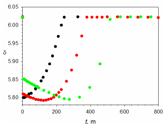
Figure 7. Controlling the duration of the conformational cycle of the calix[4]arene scaffold of 2 (4.0 mM) by regulating the excess of fuel 1,H (4.0 mM black trace, 5.4 mM red trace, 8.0 mM green trace). ^1\text{H} NMR monitoring of the chemical shift of protons on the amino-substituted aromatic rings ( \text{CD}_2\text{Cl}_2 25 °C). For related sequences of ^1\text{H} NMR spectra see Figure 3 and SI, pages S13–S14.
