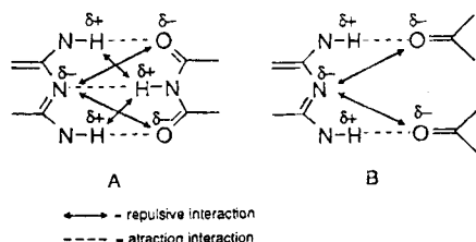
Scheme 2. Schematic representation of the association patterns of H-bonded assemblies of 1a
