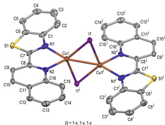
Fig. 1. View of the molecular structure of [Cu(qbtz)(μ-I)] 2 ( 1 ) with 50% probability ellipsoids. Hydrogen atoms and additional sites for the orientation-disordered qbtz ligand are omitted for clarity.
