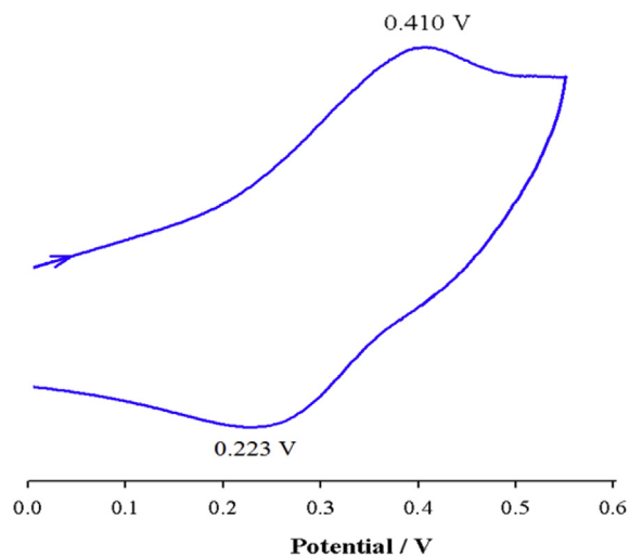
Fig. 8. Cyclic voltammogram of [\text{Cu}(\text{qbtz})(\mu\text{-SCN})] in DMF at 298 K (scan rate = 100 \text{ mV s}^{-1} , c = 5 \times 10^{-4} \text{ M} ).
