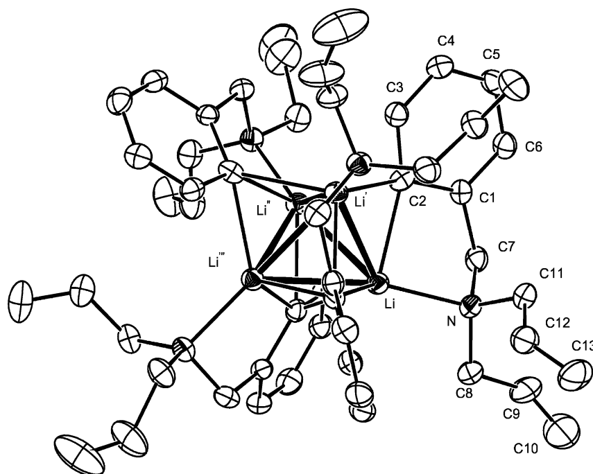
Fig. 1. The molecular structure of [\text{LiC}_6\text{H}_4\text{CH}_2\text{N}(\text{CH}_2\text{CH}=\text{CH}_2)_2]_4 ( III ), showing the atom labelling scheme.
