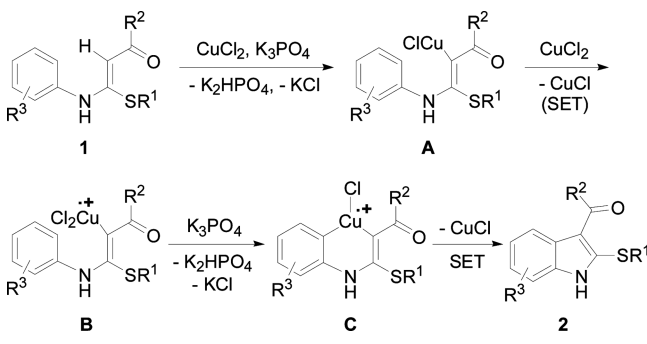
Scheme 4. Proposed Mechanism
