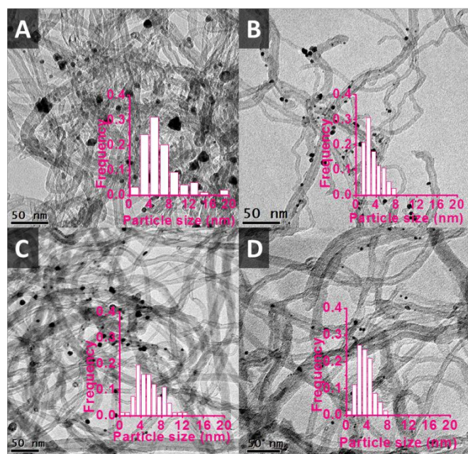
Figure 5 TEM pictures of Au-Pd alloy nanoparticles supported on various functionalised CNTs. A: AuPd/CNTs-O, average size = 6.2 nm; B: AuPd/CNTs-N, average size = 3.3 nm; C: AuPd/CNTs-S, average size = 5.2 nm; D: AuPd/CNTs-NS, average size = 3.5 nm.
