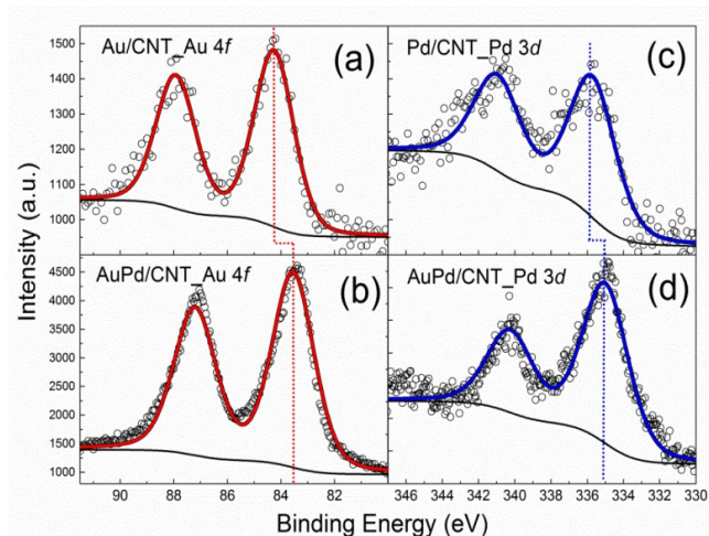
Figure 2 XPS signals of the Au 4f core level region for (a) Au/CNTs, (b) AuPd/CNTs, and of the Pd 3d core level region for (c) Pd/CNTs, (d) AuPd/CNTs.
