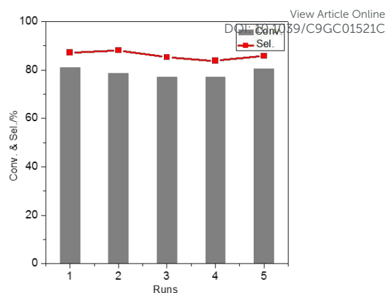
Figure 7. Catalyst recycling experiments in a batch set-up using a catalytic system consisting of AuPd/CNTs-NS and Sn-MCM-41-XS. Reaction conditions: 0.25 M glycerol in 20 ml methanol; 0.1 g of AuPd/CNTs-NS; 0.2 g of Sn-MCM-41-XS; 140 °C; 30 bar air; 4.5 h.
