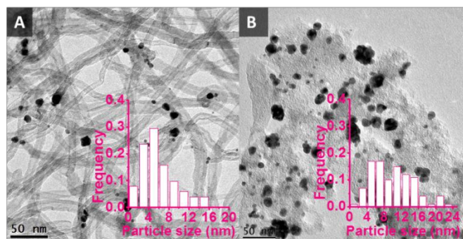
Figure 1 TEM pictures of bimetallic Au-Pd supported catalysts on unmodified CNTs and AC. A: AuPd/CNTs, average size = 6.0 nm; B: AuPd/AC, average size = 9.9 nm.
