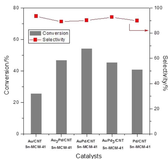
Figure 4 Performance of the catalytic system consisting of mono- or bimetallic Au-Pd on unmodified CNTs (with different Au/Pd values) and Sn-MCM-41-XS. Reaction conditions: 0.25 M glycerol in 20 ml methanol; 0.1 g of AuPd/CNTs; 0.2 g of Sn-MCM-41-XS; 140 °C; 30 bar air pressure; 4.5 h batch time.
