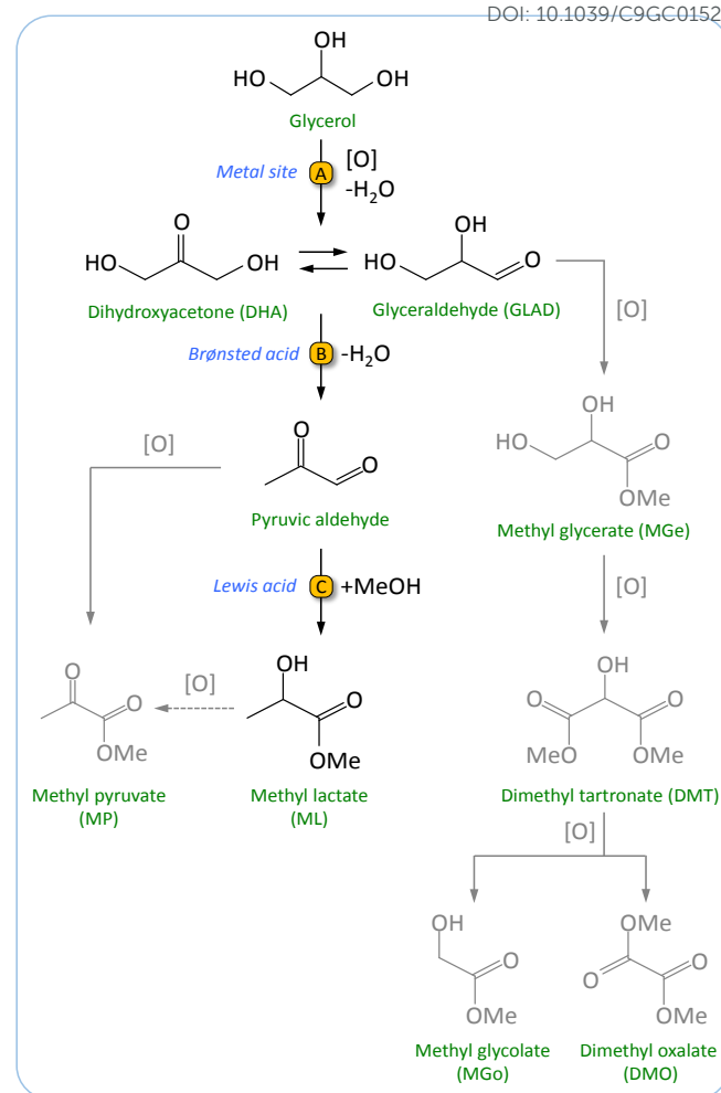
Scheme 1. Catalytic route from glycerol to methyl lactate (ML) and, in grey, the possible side-products.
