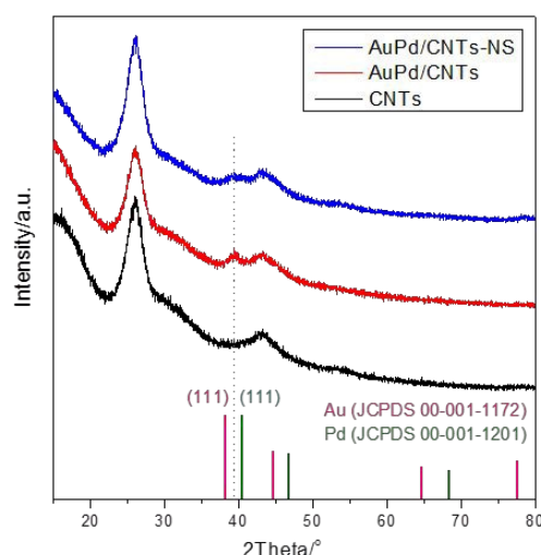
Figure 3 XRD patterns of CNTs before and after loading Au-Pd nanoparticles.
