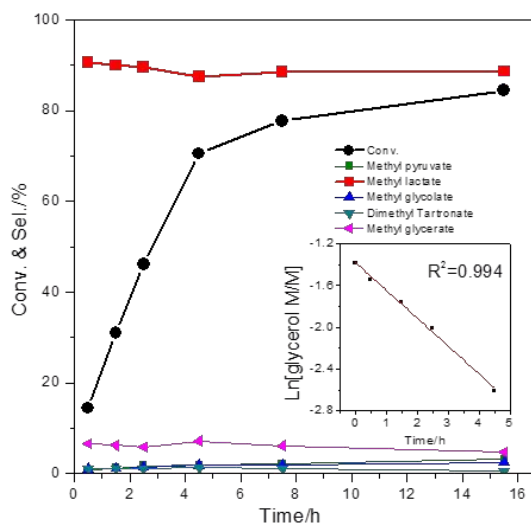
Figure 6 Glycerol conversion and product selectivity as a function of batch time for a catalyst system consisting of AuPd/CNTs-S and Sn-MCM-41-XS. Reaction conditions: 0.25 M glycerol in 20 ml methanol; 0.1 g AuPd/CNTs-S; 0.2 g of Sn-MCM-41-XS; 140 °C; 30 bar air.
