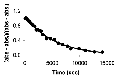
Figure 9. Kinetic data for hydrolysis of p -nitrophenyl phosphate promoted by \text{Cp}'_2\text{Mo}(\text{OH})(\text{OH}_2)^+ fit to the exponential equation y = 1.06e^{-1.87 \times 10^{-4}x} , R^2 = 0.992 .
