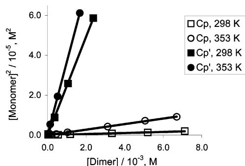
Figure 3. Plots of [\text{CpR}_2\text{Mo}(\text{OH})(\text{OH}_2)]_2[\text{OTs}]_2 versus [\text{CpR}_2\text{Mo}(\mu\text{-OH})_2][\text{OTs}]_2 in 0.13 M MOPS \text{D}_2\text{O} solution (pD 6.8). For \text{R} = \text{H} , ( \square ) K_{\text{eq}} = (2.7 \pm 0.1) \times 10^{-4} M at 25 °C and ( \circ ) K_{\text{eq}} = (1.4 \pm 0.2) \times 10^{-3} M at 80 °C. For \text{R} = \text{Me} , ( \blacksquare ) K_{\text{eq}} = (2.5 \pm 0.1) \times 10^{-2} M at 25 °C and ( \bullet ) K_{\text{eq}} = (3.7 \pm 0.3) \times 10^{-2} M at 80 °C.
