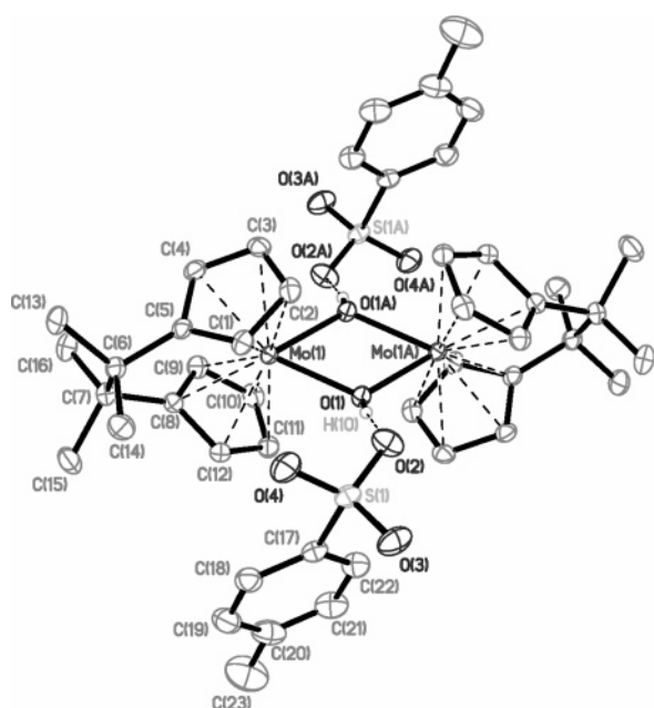
Figure 6. X-ray crystal structure of [\{\text{C}_2\text{Me}_4(\text{C}_5\text{H}_4)_2\}\text{Mo}(\mu\text{-OH})]_2[\text{OTs}]_2 (5). The H atoms were omitted for clarity. Thermal ellipsoids are drawn at the 50% probability level.
