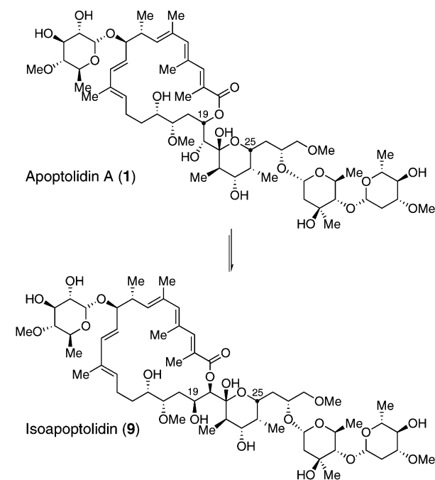
1 H NMR Comparison of Apoptolidin and Analogues
