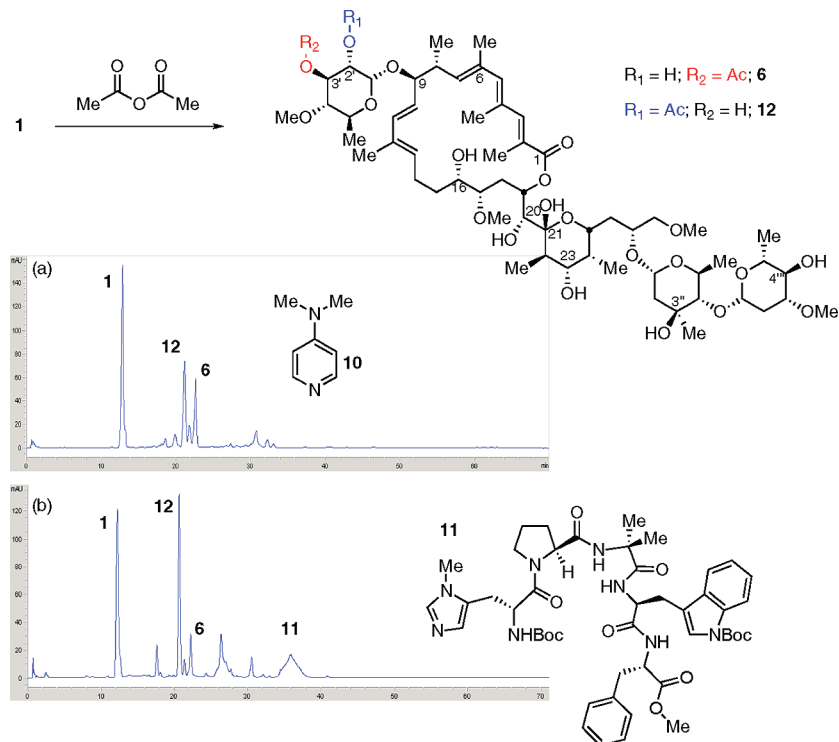
Figure 1. Low-conversion reactions of apoptolidin A (1). (a) Reversed-phase HPLC trace of the reaction mixture when 10 is employed as the catalyst. (b) Reversed-phase HPLC trace of the reaction mixture when 11 is employed as the catalyst.
