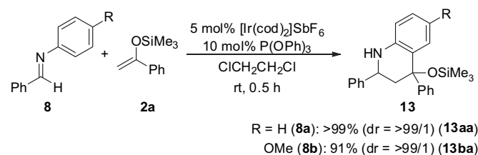
Scheme 6. The reaction of aldimine 8 with silyl enol ether 2a .
