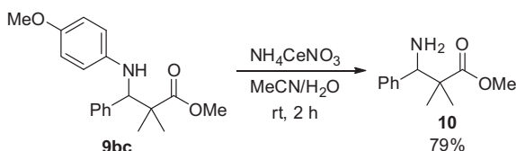
Scheme 3. Deprotection of 9bc .
