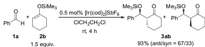
Scheme 1. The reaction of benzaldehyde ( 1a ) with 2b .
