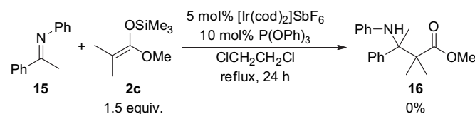
Scheme 8. The reaction of ketimine 15 with ketene silyl acetal 2c .
