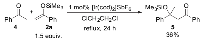
Scheme 2. The reaction of ketone ( 4 ) with 2a .
