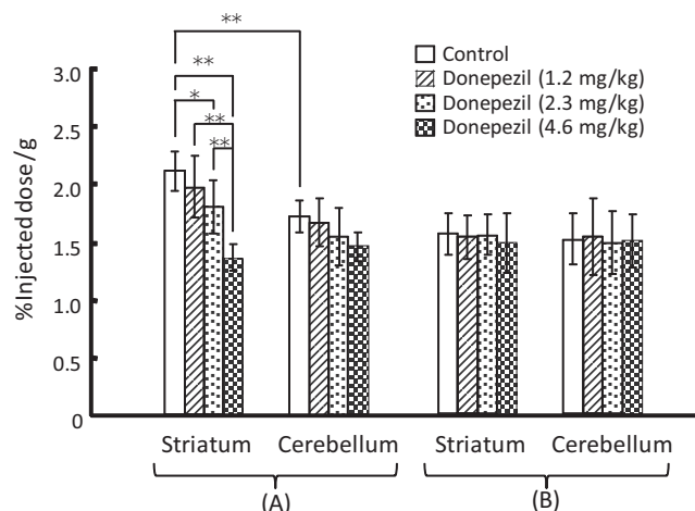
Figure 3. Effect of different dosages of donepezil on the uptake of (–)-[ 11 C]galanthamine (A) and (+)-[ 11 C]galanthamine (B) in two brain regions of mice. Both (–) and (+)-[ 11 C]galanthamine were administered intravenously (iv), 30 min after iv donepezil treatment [where * p < 0.05; ** p < 0.01 (vs control)].
