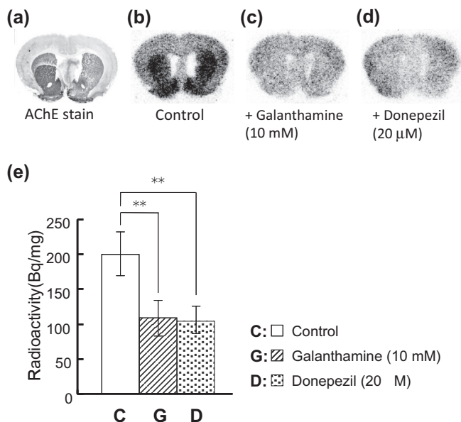
Figure 4. Accumulation of (–)-[ 11 C]galanthamine in rat brain sections as determined by in vitro autoradiography, with: AChE staining of a rat coronal brain section; (a) representative in vitro autoradiograms of rat coronal brain sections at 30 min after incubation of (–)-[ 11 C]galanthamine; (b), with galanthamine (10 mM); (c) or donepezil (20 μM); (d) illustration of the significant decrease in accumulation of (–)-[ 11 C]galanthamine in the presence of galanthamine or donepezil; (e) (where ** p < 0.01 vs control).
