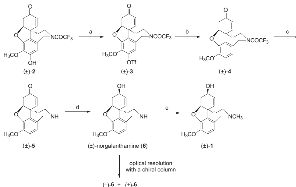
Scheme 1. Reagents and conditions: (a) \text{TiF}_4 , pyridine, 0 °C, 91%; (b) \text{Pd}(\text{OAc})_2 , dppe, \text{Et}_3\text{N} , \text{HCO}_2\text{H} , DMF, 60 °C, 97%; (c) \text{NaOH} , MeOH, rt, 98%; (d) L-Selectride, THF, –78 °C to rt, 84%; (e) (method A) \text{HCHO} , \text{NaBH}_3\text{CN} , \text{CH}_3\text{CO}_2\text{H} , rt, 5 min, 92%, (method B) \text{CH}_3\text{OTf} , \text{Cs}_2\text{CO}_3 , DMSO, 170 °C, 5 min, 33%.
