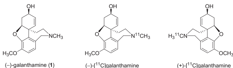
Figure 1. Chemical structures of (–)-galanthamine, (–)- and (+)-[ 11 C]galanthamine.
