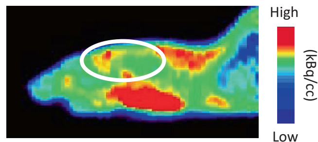
Figure 5. Sagittal PET image of (–)-[ 11 C]galanthamine in the ddY mouse. The region surrounded by the ellipse indicates the location of the brain.
