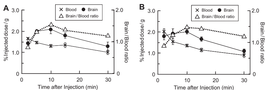
Figure 2. Brain and blood levels of (–)- [^{11}\text{C}] galanthamine (A) and (+)- [^{11}\text{C}] galanthamine (B) in ddY mice. Values representing % injected dose/gram tissue are means \pm sd ( n = 5 ). The brain/blood ratios are also shown (broken line).
